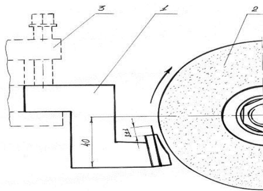
Fig.1 Experimental installation for preparing thin lamellar knives for work. 1- knife holder; 2- sharpening shaft; 3- machine cutter holder.
