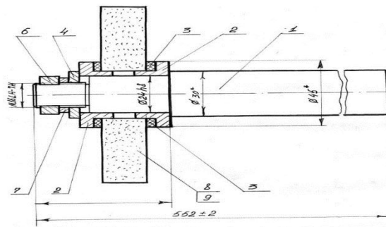
Fig. 2. Sharpening shaft of the experimental installation.
