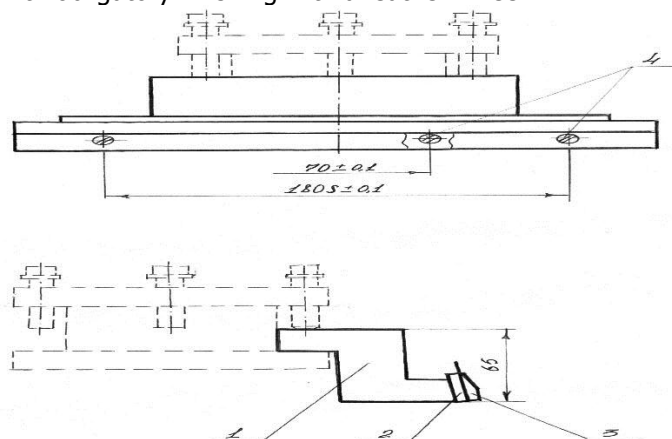
Fig. 3. Knife holder: 1- case; 2- body plate; 3- consignment plate; 4- screws.
