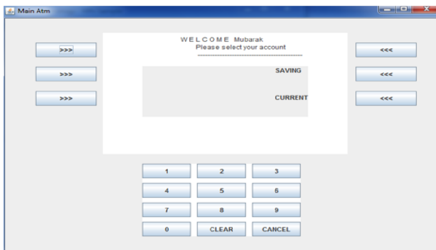
Figure 4: Transaction Page
