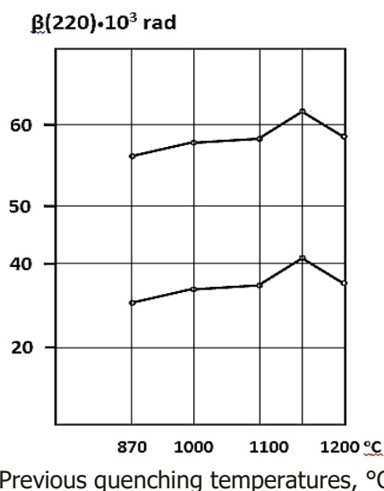
Fig. 1. Change in the parameters of the structure of steel U8A depending on the previous quenching and medium tempering.
