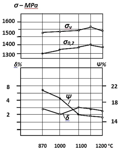
Previous quenching temperatures. °C
