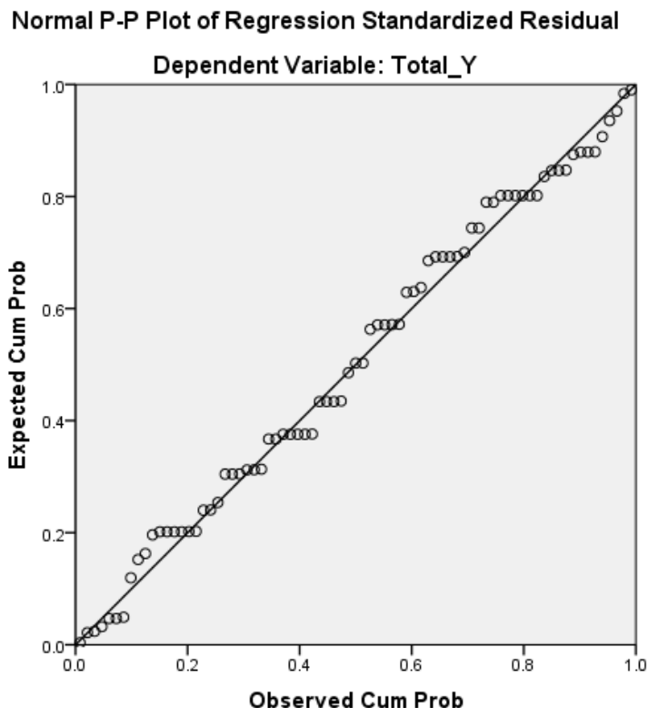
Figure 1 Normality Test
