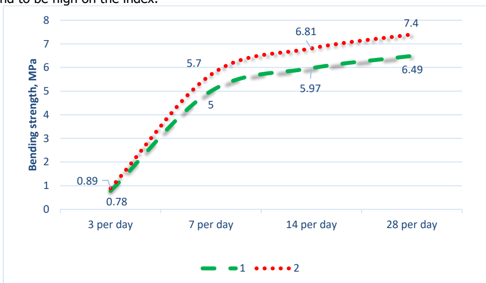
Figure 2. Bending strength of standard (1) and complex-modified (2) components
