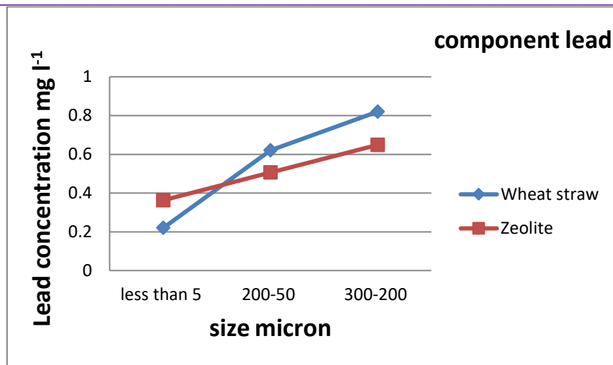
Fig .1.The effect of zeolite and wheat straw minute sizes on the adsorption of the lead element from wastewater.
