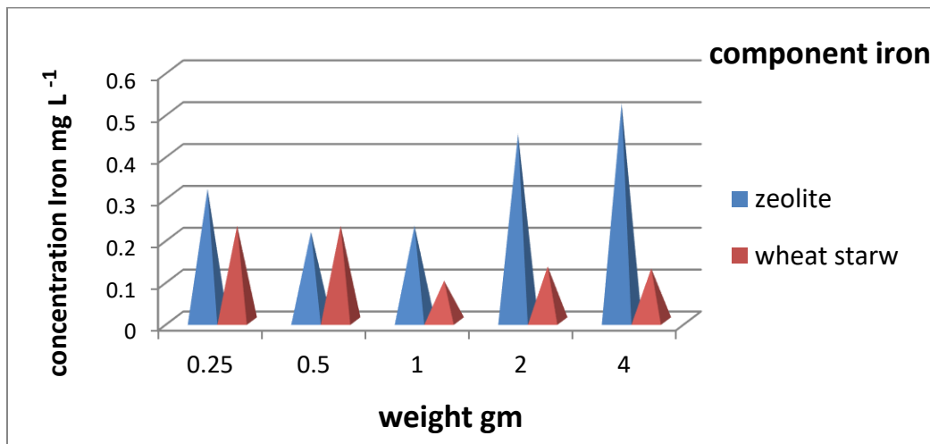
Fig.7. The effect of zeolite and wheat straw minute weight on the adsorption of the Iron element from wastewater
